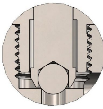
Non-rotating Ball Tip
