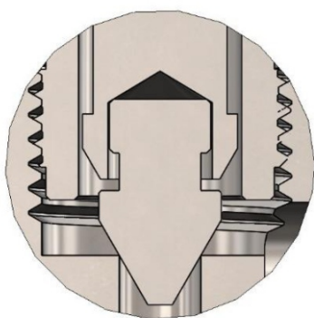
Non-rotating V Tip
