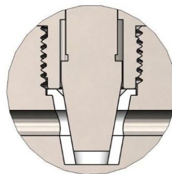
Soft Seat-large bore
