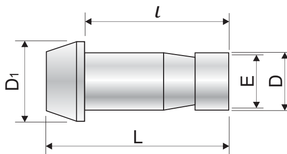
Connects metric tube
